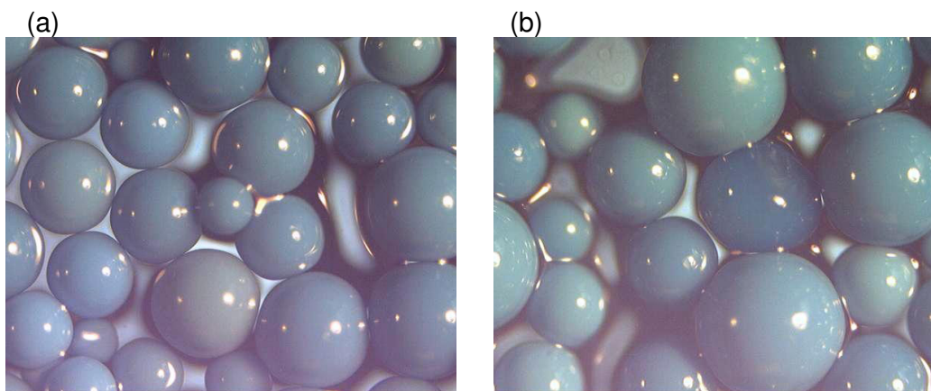
Fig.6a-b. Lewatit TP 207 (a) and Lewatit TP 208 (b) after 50 cycles of Cu(II) ions sorption-desorption process (magnification 40x).
