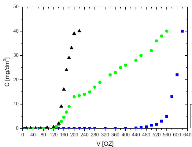
Fig.8a-b. The breakthrough curves of Cu(II), Zn(II) and Ni(II) ions at pH=2 (a) and pH=4 (b) on chelating ion exchanger Lewatit TP 207 in the \text{Na}^+ form (NaCl concentration 40 \text{ g/dm}^3 ).
