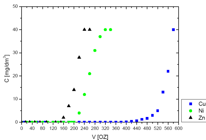
Fig.9a-b. The breakthrough curves of Cu(II), Zn(II) and Ni(II) ions at pH=2 (a) and pH=4 (b) on chelating ion exchanger Lewatit TP 207 in the \text{Na}^+ form ( \text{NaCl} concentration 40 \text{ g/dm}^3 ).
