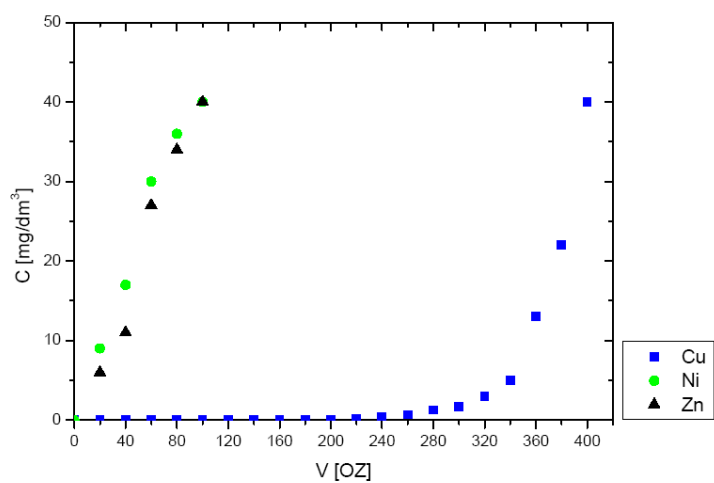
Fig.7a-b. The breakthrough curves of Cu(II), Zn(II) and Ni(II) ions at pH=2 (a) and pH=4 (b) on chelating ion exchanger Lewatit TP 207 in the \text{H}^+ form (NaCl concentration 40 \text{ g/dm}^3 ).
